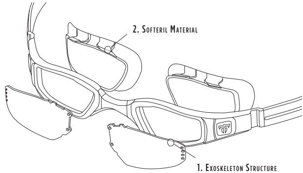
EXPANDED VIEW OF NINJA GOGGLE
