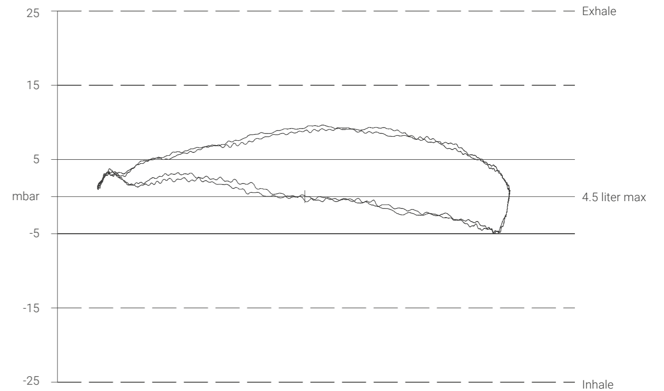
Pressure - Volume Diagrams at Mean Depth of: 51.9 msw (170.4 fsw)
